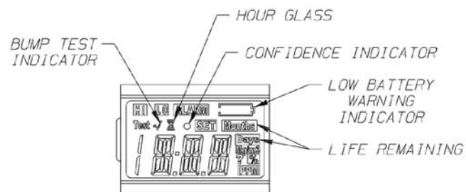
Figure 2-2. Altair Display
